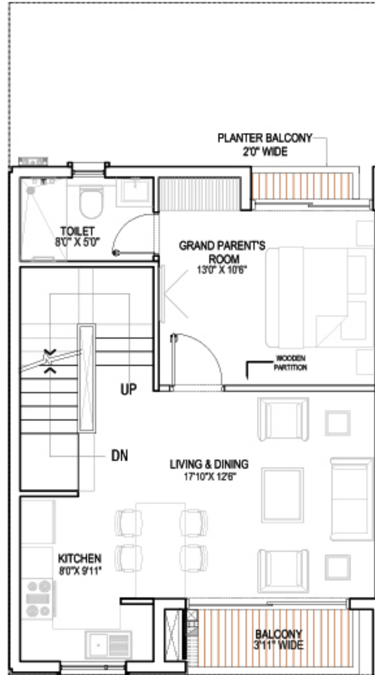
UPPER GROUND FLOOR PLAN
