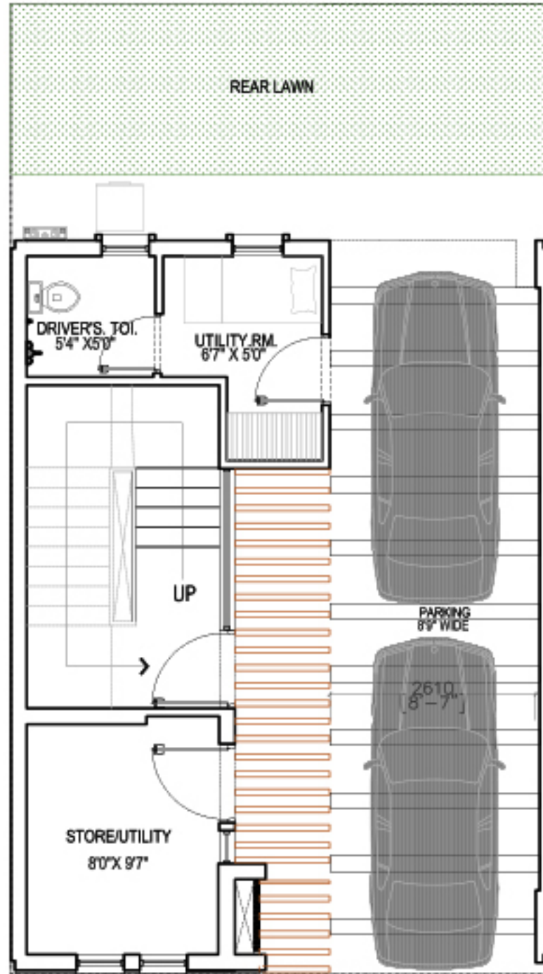
STILT LEVEL PLAN
